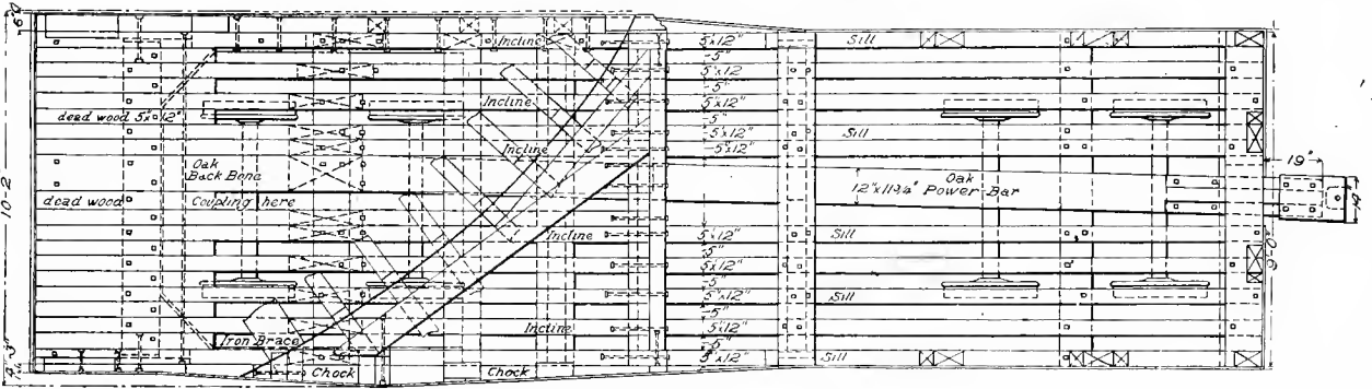
Fig. 409. Plan of Framing.
